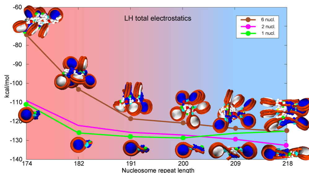
Figure 7. Chromatin structures vs electrostatic energy for mononucleosomes, dinucleosomes, and 6-core arrays over NRLs most commonly encountered in living cells. Representative images correspond to selected points on the energy curves. Mononucleosomes and dinucleosomes are electrostatically the most stable nucleosome arrays with strongest electrostatic attractions for a given NRL (green and pink curves respectively). The 6-core arrays are closest to chromatin in vivo. Genetically active cells have loosely bound LHs that interact asymmetrically with one DNA linker only. Mature, transcriptionally inactive cells have LHs tightly bound to parental DNA linkers and thus serve as barriers to transcription. The background gradient represents biological activity of chromatin over different NRLs, from chromatin in genetically active cells with high protein production in red to mature eukaryotic cells with limited protein production in light blue.
