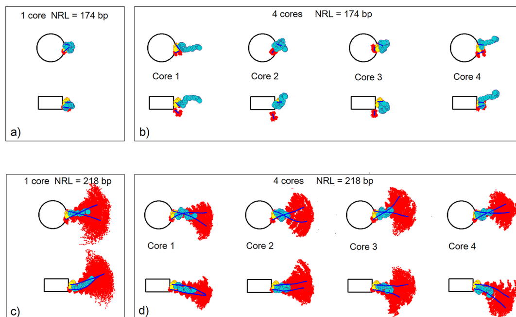
Figure 5. Linker DNA distributions for typical fiber configurations in mononucleosomes and 4-nucleosome arrays, for shortest (174 bp) and longest (218 bp) NRLs, projected on the nucleosome and dyad plane. The mean trajectories of the DNA linkers are shown as blue lines. The clouds of red dots represent linker DNA positions sampled throughout a single trajectory. The average positions of linker histone beads are shown as yellow (GH) and turquoise (CTD) circles.
