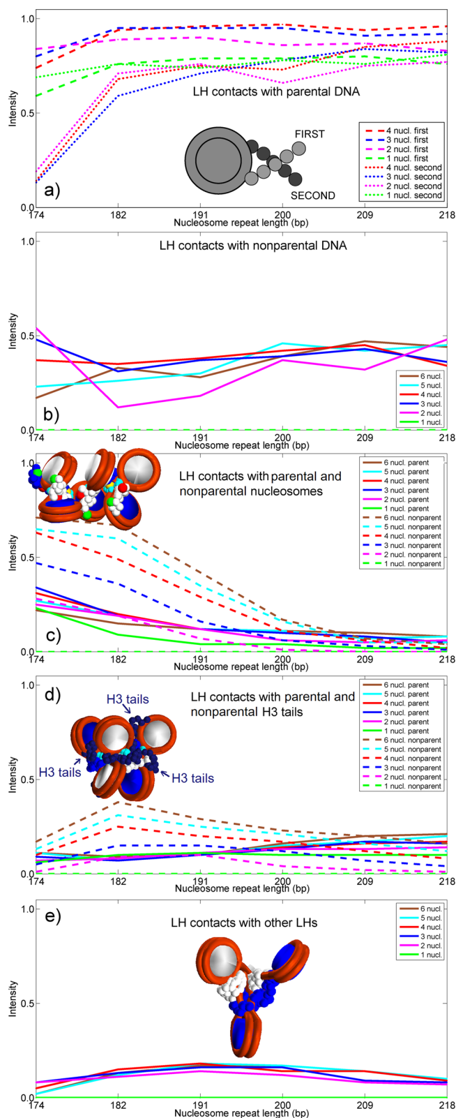
Figure 2. LH interactions with parental and nonparental DNA linkers, nonparental cores, H3 tails, and nonparental LHs. Intensities are counted in a binary manner (on or off) when distances are within half the sum of van der Waals radii of LH (1.8 Å) and other elements (1.8 Å for tails and 2.7 Å for DNA). Total values are normalized. (a) LH interactions with first parental (---) and second parental DNA linkers (···). (b) LH interactions with nonparental DNA. (c) LH interactions with parental (—) and nonparental nucleosomes (---). (d) LH
