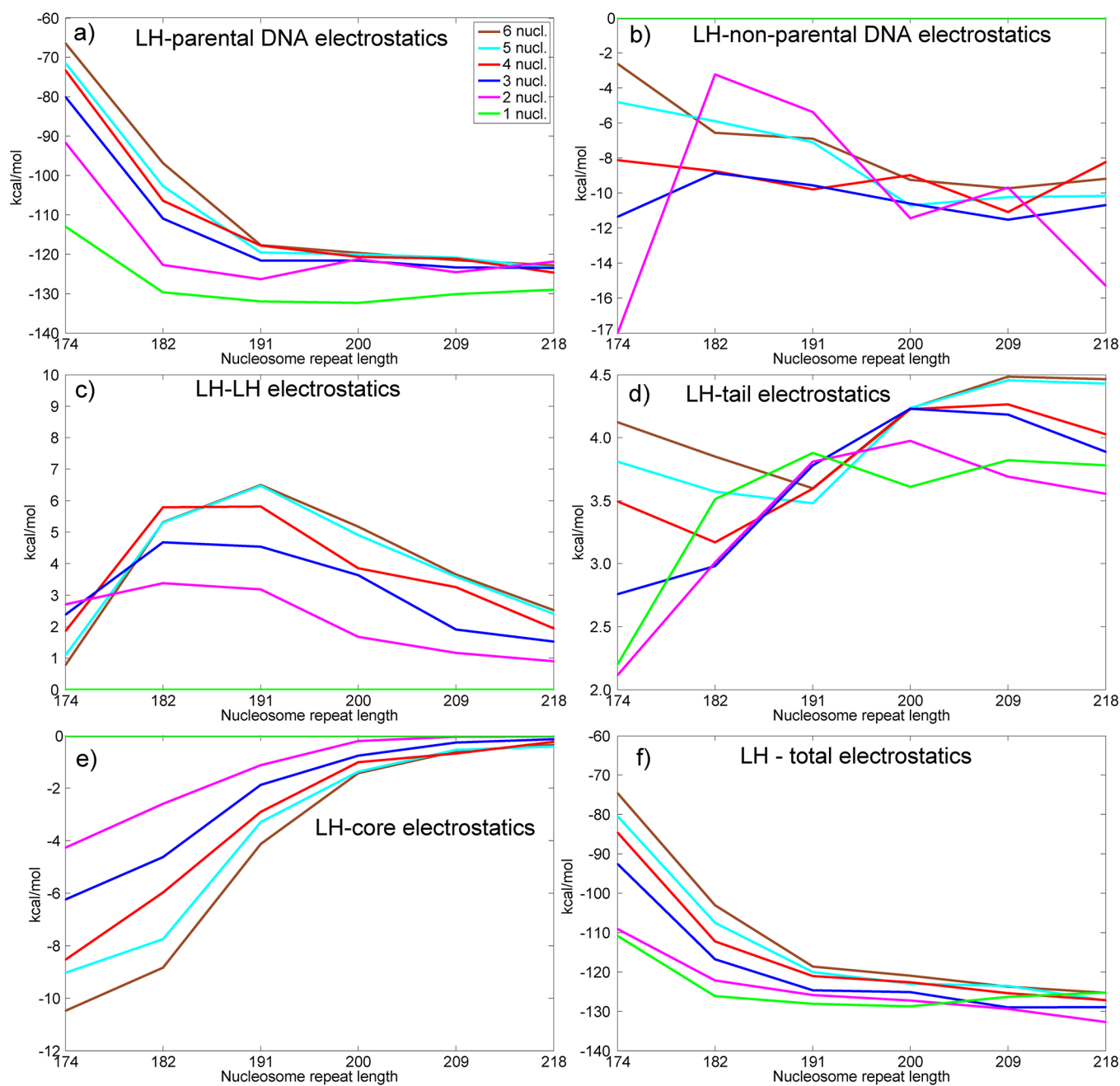
Figure 3. Array electrostatics. Average electrostatic energies per nucleosome in the chromatin arrays are measured in kcal/mol. (a) Electrostatic energy between linker histone and parental DNA strands. (b) Electrostatic energy between linker histone and nonparental DNA strands. (c) Electrostatic energy among all linker histones. (d) Electrostatic energy between linker histone and tails. (e) Electrostatic energy between linker histone and nucleosome core(s). (f) Total electrostatic energy.
