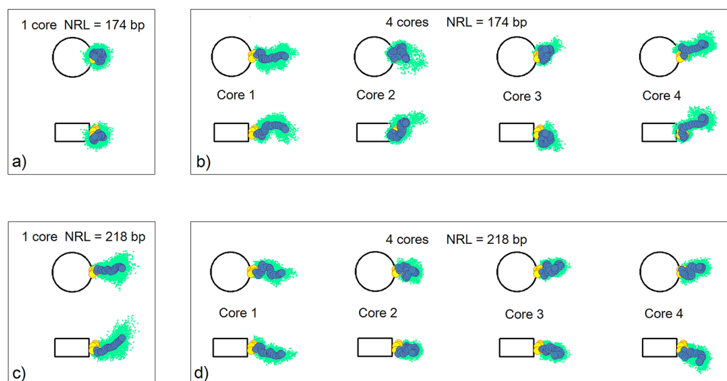
Figure 4. Linker histone distributions for typical fiber configurations in mononucleosomes and 4-nucleosome arrays, for shortest (174 bp) and longest (218 bp) NRLs, projected on the nucleosome and dyad planes. The clouds of light green dots represent linker histone positions sampled throughout a single trajectory. The average positions of linker histone beads, for a given trajectory, are shown as yellow (GH) and blue (CTD) circles.
