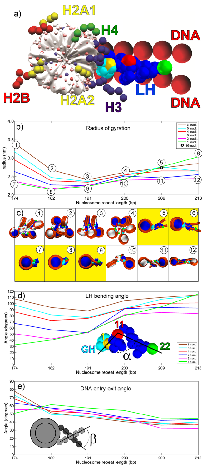
Figure 1. Chromatin-dependent condensation of LH. (a) Our mesoscale model of nucleosome core with tails, DNA linkers, and LH. (b) Linker histone radius of gyration as a function of the number of nucleosomes in the array and NRL. Radius of gyration data for 96-core array (NRL = 207 bp) taken from ref 35. (c) Configurations associated with lowest LH condensation/ highest gyration radii (upper panels) and highest LH condensation/lowest gyration radii (lower panels) for each NRL. LHs have the same colors as their parent nucleosomes (consecutive nucleosomes are colored white and blue). GH is colored cyan. The first bead in CTD is colored yellow. Bead 11 is colored red, and the last bead (22) is green. Mononucleosomes are in yellow boxes. (d) CTD bending angle (angle between vectors formed by beads 1–11 and 11–22). (e) Angle between DNA linkers
