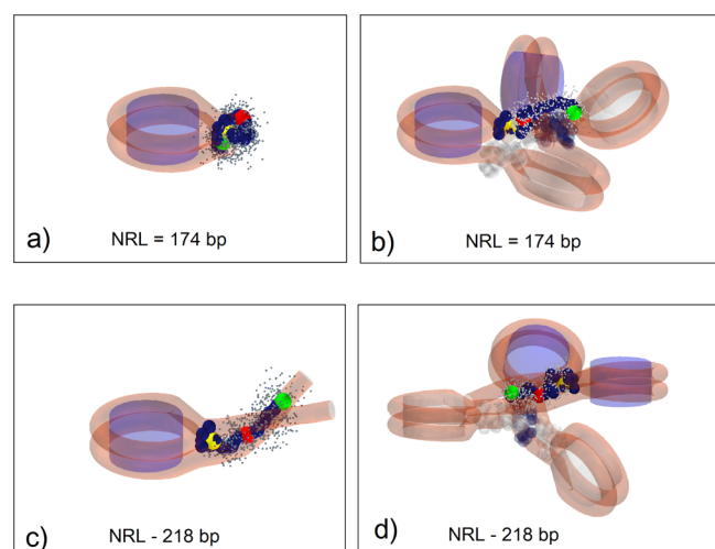
Figure 6. Three-dimensional CTD distributions for typical fiber configurations in mononucleosomes and 4-nucleosome arrays, for shortest (174 bp) and longest (218 bp) NRLs. Each image depicts an average configuration of one LH over the last 5 million steps per a single trajectory. All other LHs are shown as semitransparent and carry the same color as their parental nucleosome (white or navy). Small gray beads are trajectory positions of CTD beads. Analyzed CTDs are opaque, navy colored, with bead 1 in yellow, bead 11 in red, and bead 22 in green. (a) Mononucleosome with NRL = 174 bp. (b) 4-Nucleosome array with NRL = 174 bp. (c) Mononucleosome with NRL = 218 bp. (d) 4-Nucleosome array with NRL = 218 bp.
