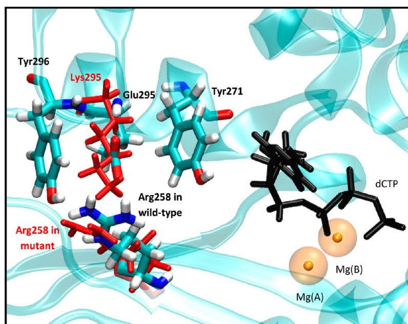
Figure 6. “Sandwich-shaped” structure formed by Glu295/Lys295, Tyr296, and Tyr271 tends to cause steric hindrance for Arg258 in the E295K mutant complex. The residues Lys295 and Arg258 (red) from the final closed form of the E295K mutant are superimposed onto the ternary crystal structure of wild-type pol \beta . Mg(A), catalytic ion; Mg(B), nucleotide-binding ion.
