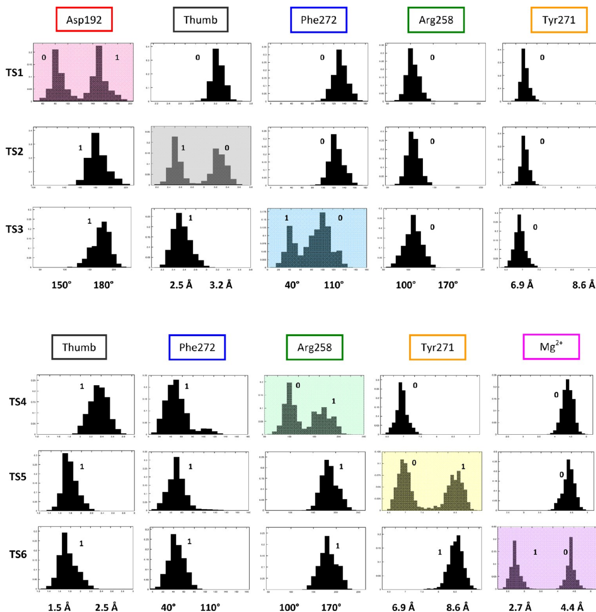
Figure 2. Normalized probability distribution of the order parameters for the transition states revealed (TS1–TS6). Labels 0 and 1 indicate the open- and closed-form conformations.
