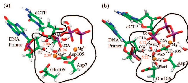
Figure 3. The catalytic sites of Dpo4 in the optimized (a) and the crystal state models (b). QM atoms are enclosed in the black circles. The missing 3'OH of the primer terminus was added using CHARMM in both models. The critical distances, namely \text{O3}'\text{--Mg}^{2+} (cat.), \text{Mg}^{2+} (cat.)– \text{O2A} , and \text{P}_\alpha\text{--O3}' (in Å) are shown by dashed lines and labeled in red.
