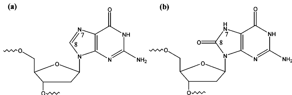
Figure 1. Molecular formulas of (a) guanine and (b) 8-oxoguanine.
